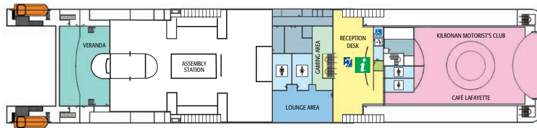
DECK 7
